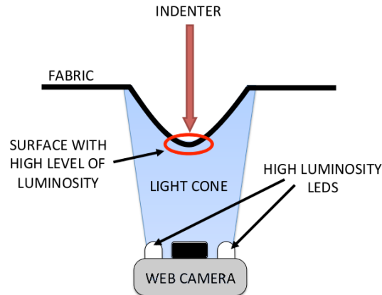
Fig. 4 The measurement of the contact area.
