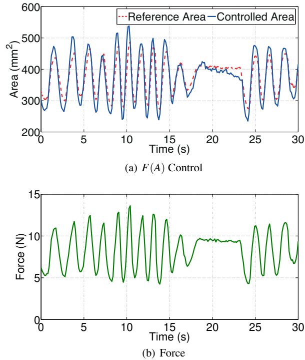
Fig. 13 Reference area (dashed line) vs. Controlled area (continuous line) (a). Force measurement (b).
