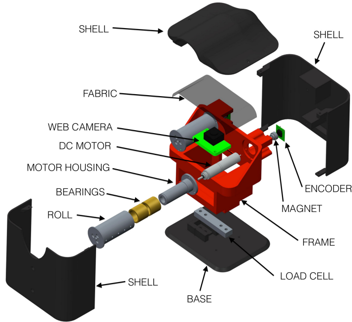
Fig. 9 FYD-2, exploded drawing view.
