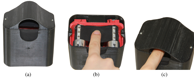
Fig. 7 The FYD-2, an overview (a). A finger interacting with the display. For the sake of clarity the FYD-2 is shown without and with the cover in (b) and in (c), respectively.
