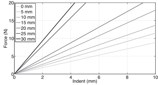
(a) Force/Indentation Characteristics
