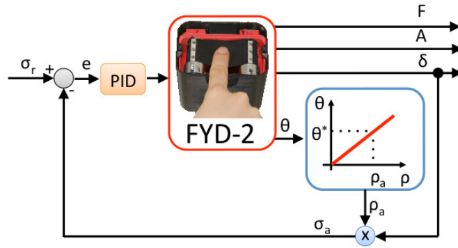
Fig. 10 The control scheme used for constant stiffness tracking . A PID control is used to control motor positions, based on the error ( e ) between \sigma_r (reference stiffness) and \sigma_a (actual stiffness).
