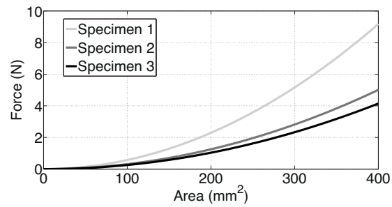
Fig. 15 The force/area ( F(A) ) characteristics for the silicone specimens.
