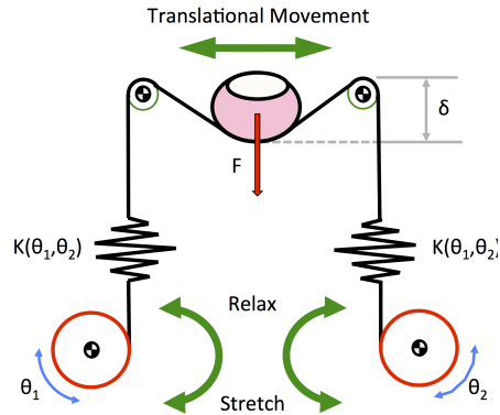
Fig. 8 How the system works during the interaction with a human finger pad. K is the stiffness of the fabric, which depends on motor positions, \theta_1 and \theta_2 .
