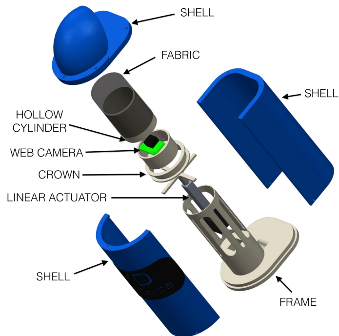
Fig. 3 The FYD first prototype: exploded drawing view.
