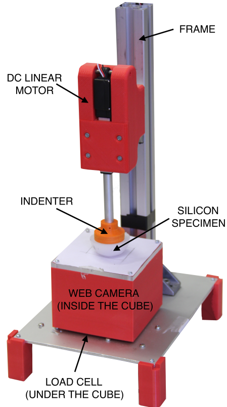
Fig. 14 The system used for the characterisation of the silicone specimens.
