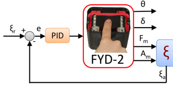
Fig. 12 The block diagram of control for F(A) curve tracking. Let be F(A) = \xi_r A_r^2 , the quadratic curve to be tracked, with \xi_r in [N/mm^4] the quadratic coefficient of the curve. In order to properly implement the control, we need to know the actual \xi_a [N/mm^4] coefficient. This coefficient is obtained each time by dividing the indenting force measured by the load cell for the squared value of the measured area A_m . F_m is the measured force. A PID controller is then used to control the quadratic coefficient.
