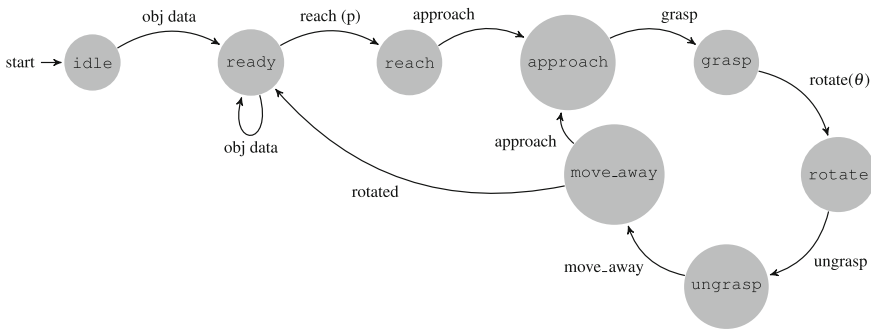
Fig. 30 Finite state machine of the valve turning task
